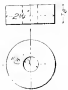
Figs. 4640-4641. CAST-WASHER.
